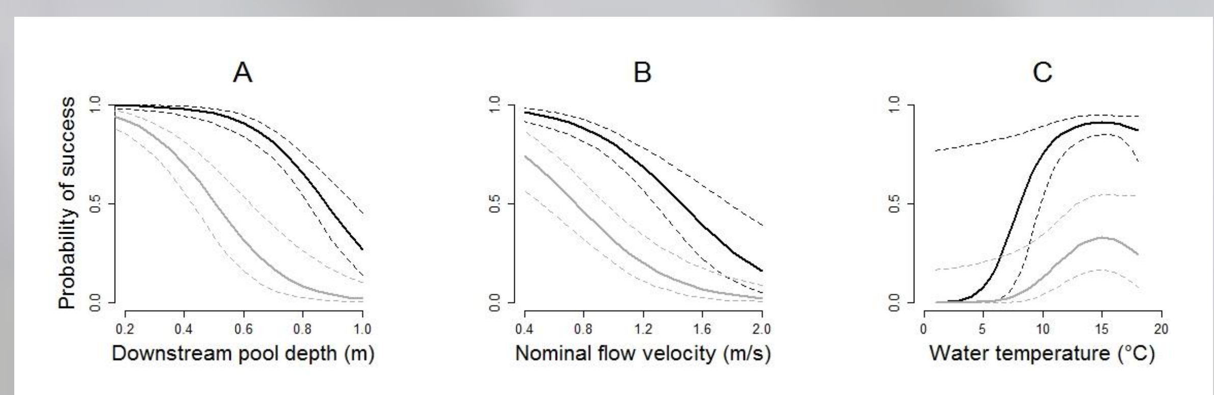
Figure 2: Probability of success with regards to downstream pool depth (A), flow velocity (B) and water temperature (C), in corrugated (black) and smooth (gray) culverts.
