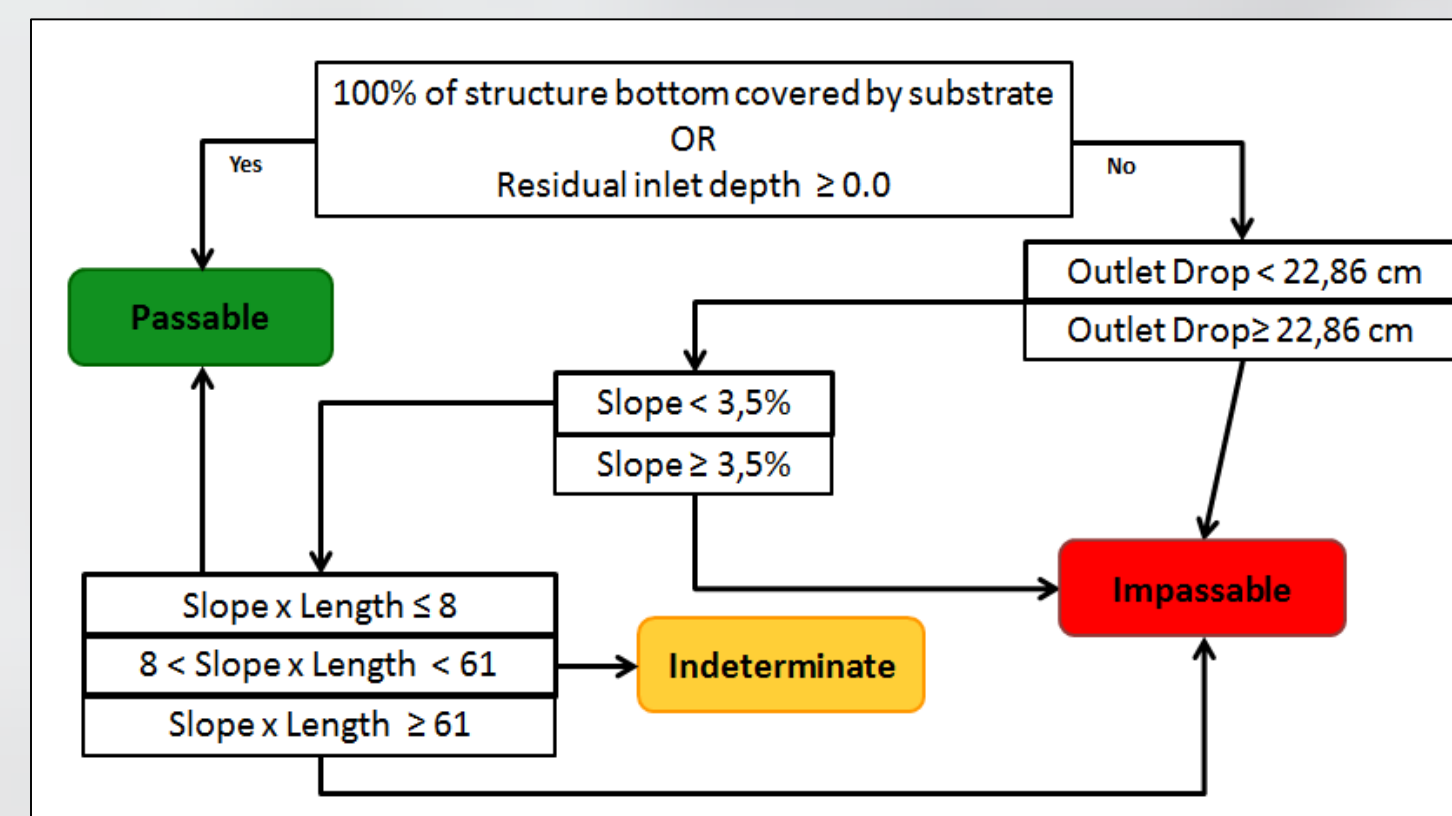
Figure 2 Coarse filter of the predictive model for upstream passage through culverts for juvenile salmonids (Coffman, 2005) classifying culverts in three categories according to threshold values of physical parameters.
