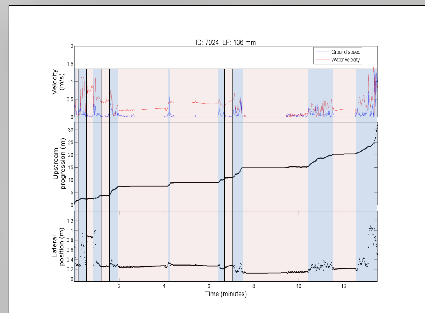
Figure 4. Example of the forward progression and lateral position of a trout in relation to the nose flow velocity experienced. Blue and red rectangles represent the movements and stops, respectively.
