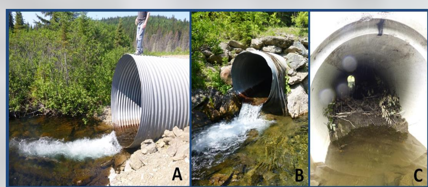
Figure 2 Coarse filter of the predictive model for upstream passage through culverts for juvenile salmonids (Coffman, 2005) classifying culverts in three categories according to threshold values of physical parameters.
