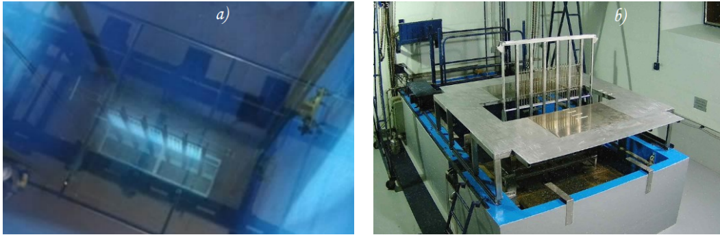
Figure 3.9. a) Calliope source rack in the pool and b) source rack within the irradiation cell (picture acquired by remote camera).
