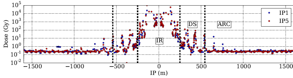
Figure 1.2. TID values during LHC 2016 proton-proton runs in IP1 and IP5 [2].
