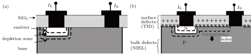
Figure 2.19. Scheme of an NPN BJT emitter base junction before (a) and after (b) irradiation [79].
