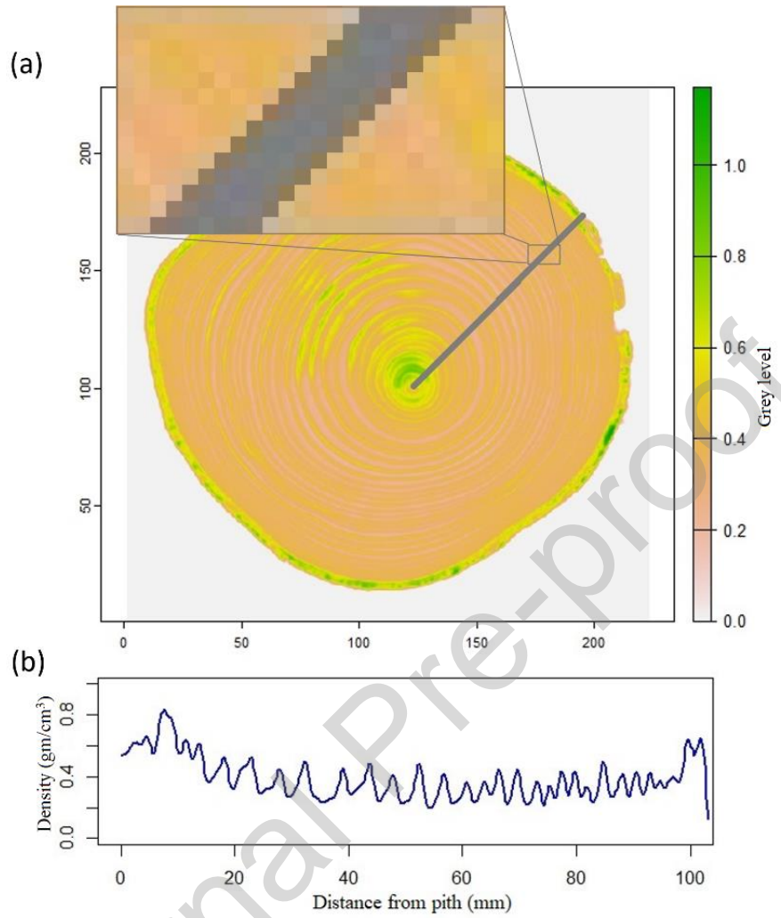
Figure 4. Profile path on the raster image, highlighting (a) the pixels through which the profile passes and (b) the plot of the profile from pith to the bark of the selected path.
