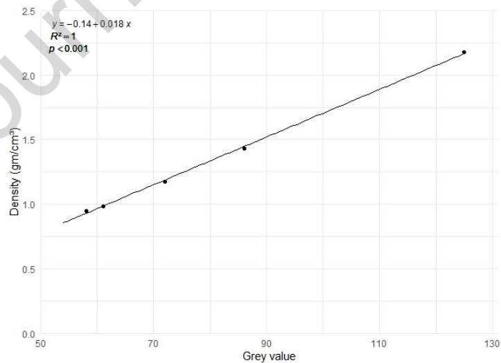
Figure 2. Calibration curve relating density to 8-bit grey values of known materials.
